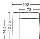
Left armrest Art. S1062 W73/102 x D74,5/103,5 x H37/67 cm Armrest D29 cm
