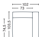
Right armrest Art. S1061 W73/102 x D74,5/103,5 x H37/67 cm Armrest D29 cm
