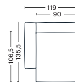
Left armrest Art. S8262 W90/119 x D106,5/135,5 x H37/67 cm Armrest D29 cm
