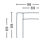
Left corner Art. S1862 W69/98 x D69/98 x H37/67 cm Armrest D29 cm
