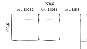
3 SEATER COMB. 9 RIGHT ARMREST
