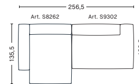
2,5 SEATER COMB. 3 LEFT ARMREST
