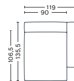
Right armrest Art. S8261 W90/119 x D106,5/135,5 x H37/67 cm Armrest D29 cm
