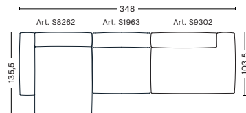
3 SEATER COMB. 5 LEFT ARMREST
