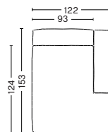
Right armrest Art. S7261 W93/122 x D124/153 x H37/67 cm Armrest D29 cm
