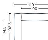
Left armrest Art. S1962 W90/119 x D74,5/103,5 x H37/67 cm Armrest D29 cm
