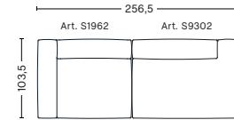
2,5 SEATER COMB. 2 LEFT ARMREST
