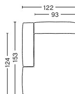
Left armrest Art. S7262 W93/122 x D124/153 x H37/67 cm Armrest D29 cm
