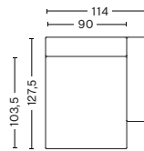
Right armrest* Art. 8261 W90/114 x D103,5/127,5 x H40/67 cm Armrest D24 cm
