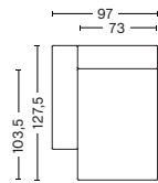
Left armrest* Art. 8162 W73/97 x D103,5/127,5 x H40/67 cm Armrest D24 cm
